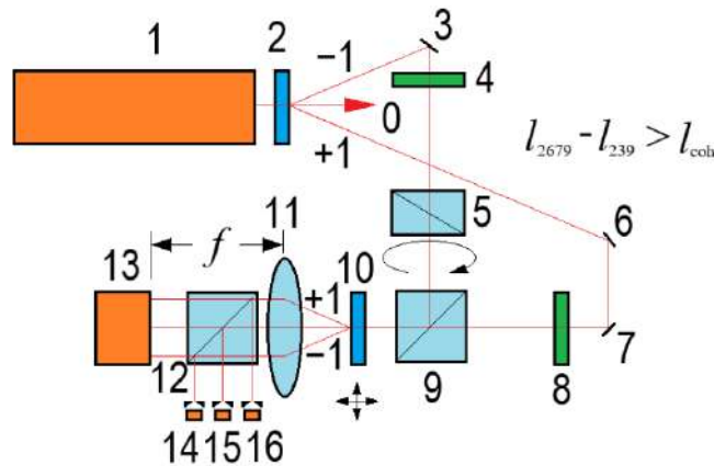
Fig. 2. Experimental setup for testing the performance of singular multiplexing
